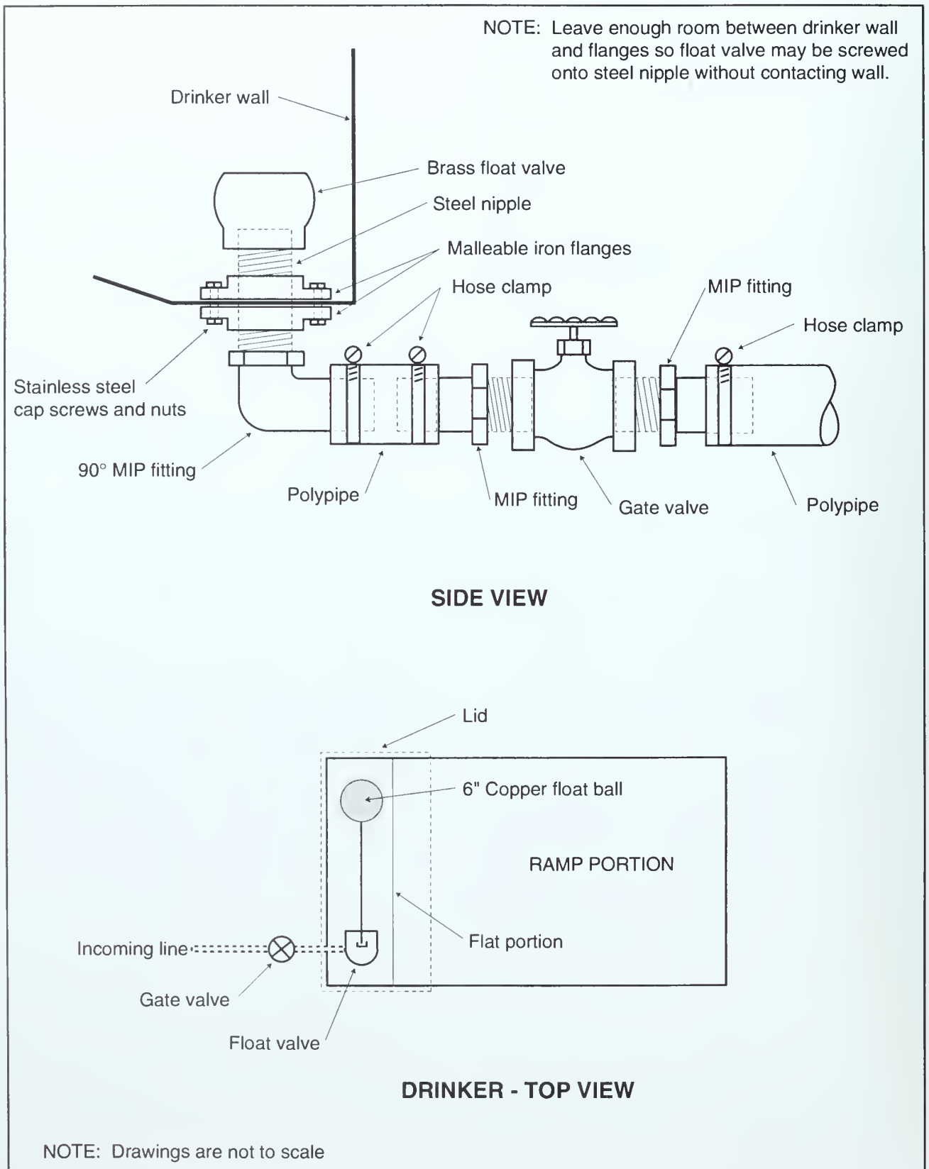
Figure 2. Float valve drinker details.
